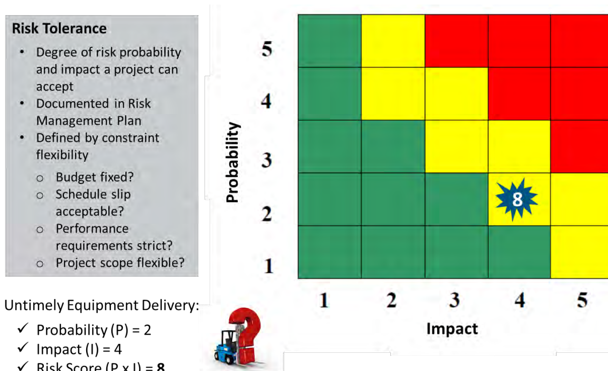
Figure 75: Risk Tolerance
